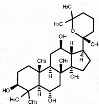
Structural Formula (1)
